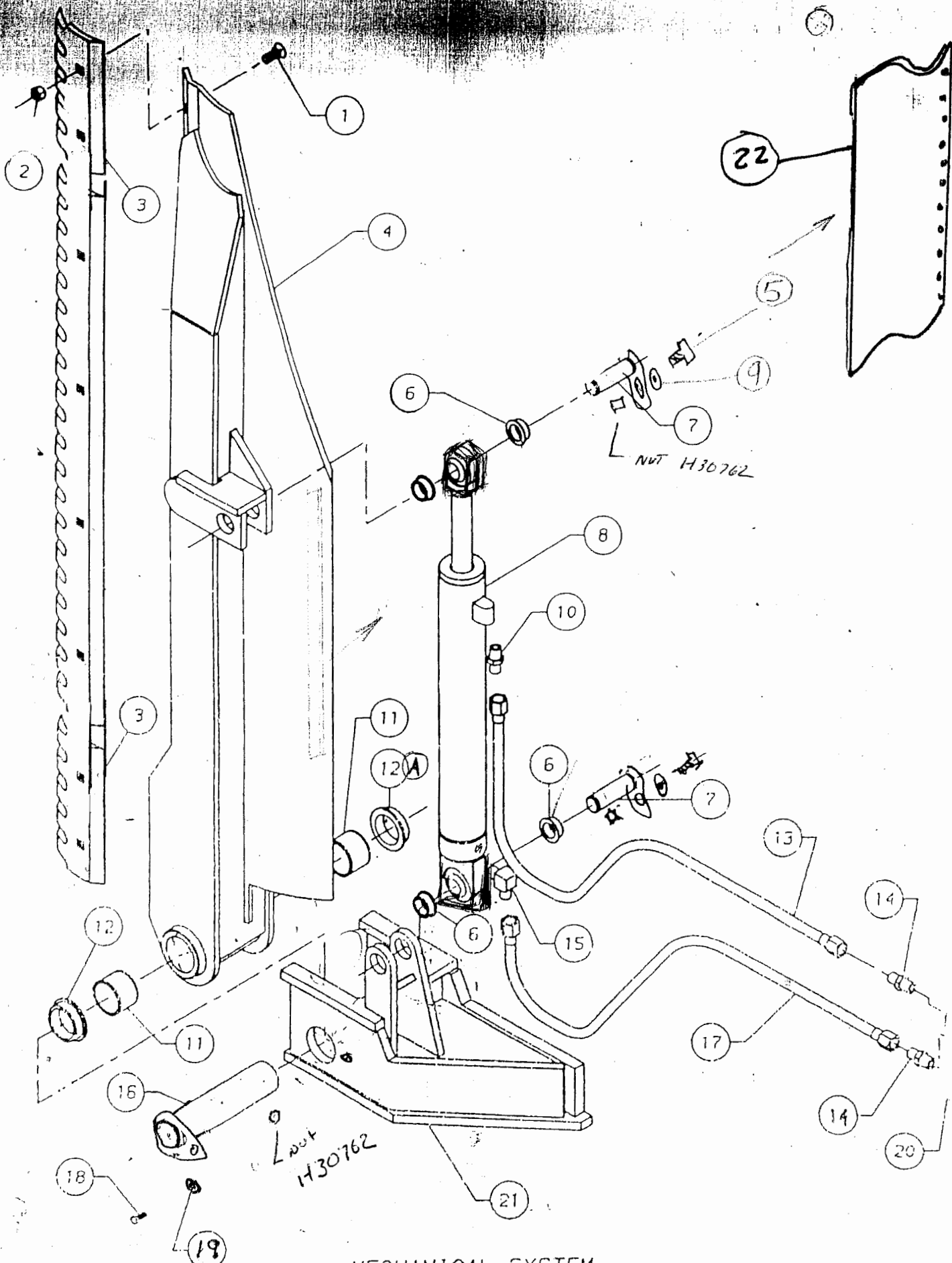
MECHANICAL SYSTEM SL5 BANK SLOPER
